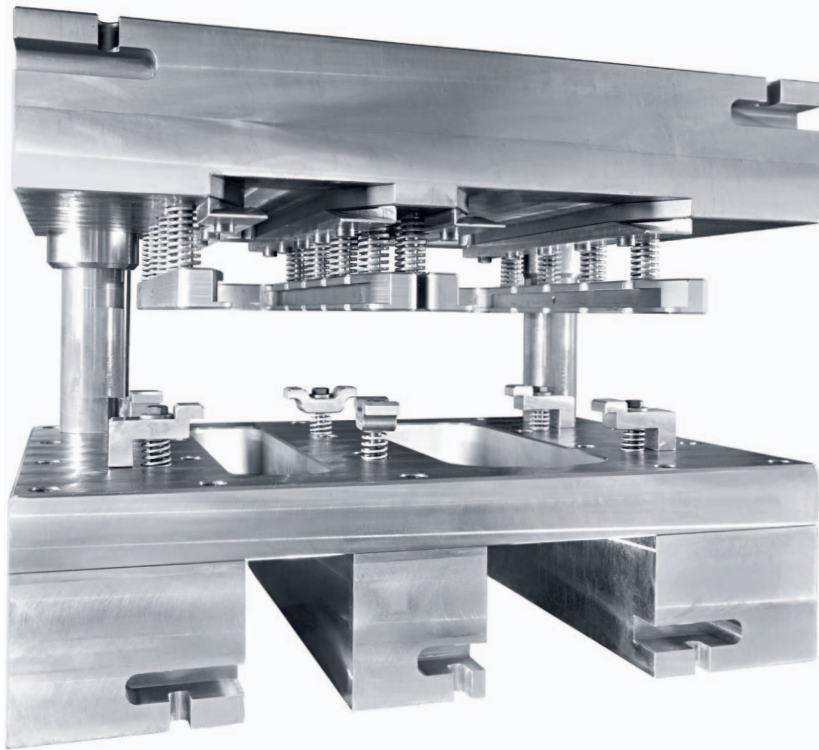
2-station trimming tool with tool round/round pillar guide and mechanical releaser, trimming tool upper section in position "press ram at top" (view from front)
