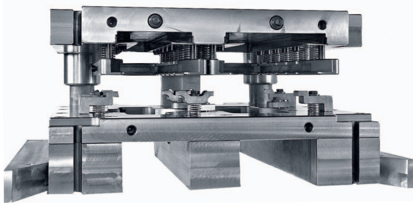
2-station cutting tool quick-change trimming tool with tool round/round pillar guide and mechanical releaser, trimming tool upper section in position "press ram in stroke centre" (view from front)
